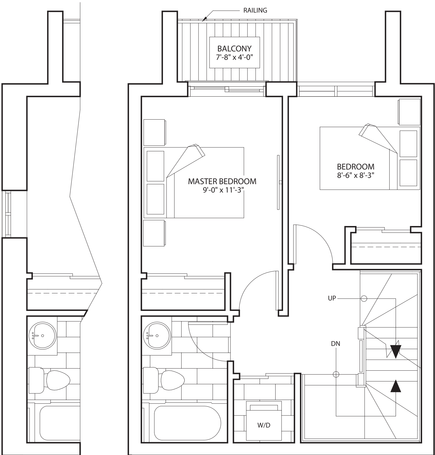
3rd Floor Enhance End Unit A
