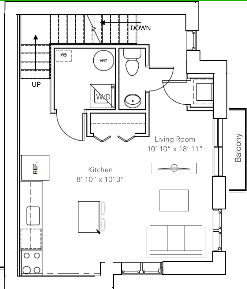
Main Level
