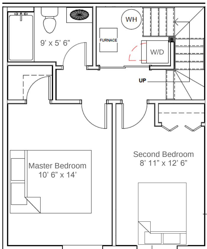
Lower Level
