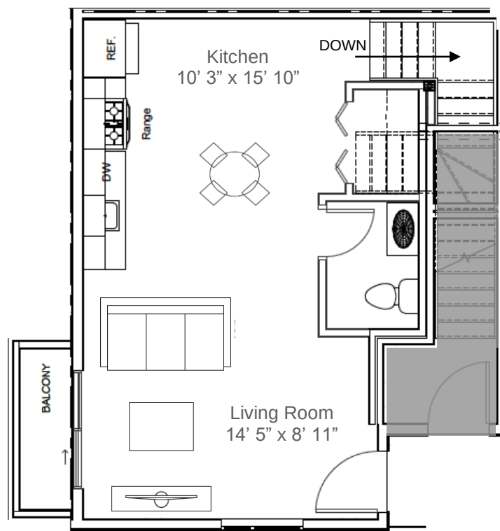
1st Floor
